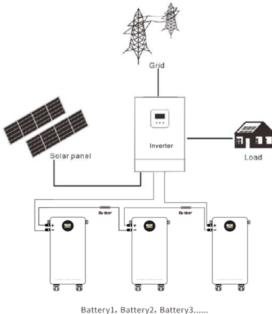
Figure 1 Operation Principle Diagram of Battery System
